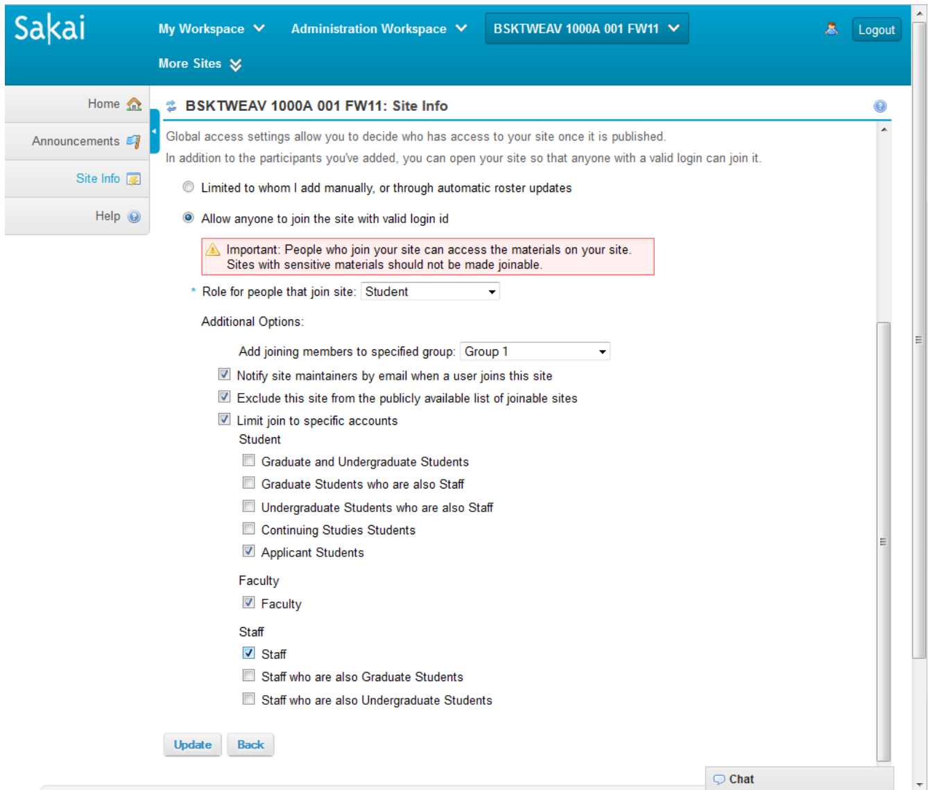
Figure 3 - All settings enabled, with previous selections
